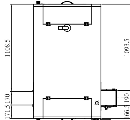
5 HP Option (選配) 77 dB (噪音分貝)
